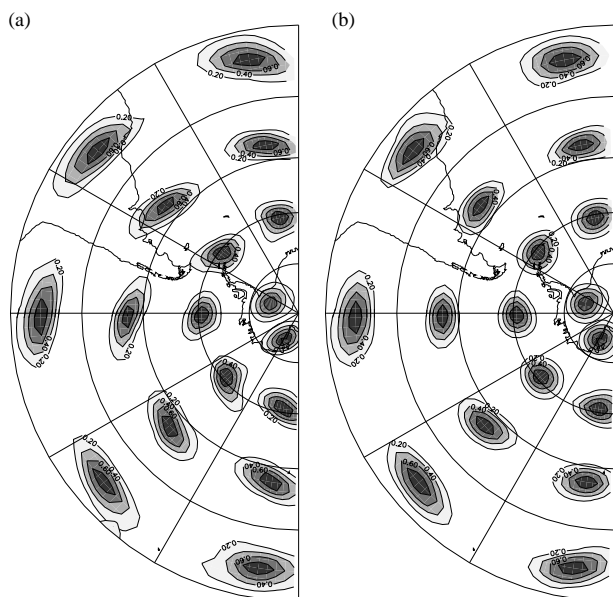
Figure 6. Examples of correlation functions of the background error viewed from the South Pole: (a) diagnosed from the ensemble of perturbed forecast and (b) from the correlation model diagnosed using a randomization method with 6400 samples. The contour lines correspond to values within the range 0.2 – 1, with an 0.2 increment. Parallel lines are plotted every 15 degrees from 90 °S to 15 °S.
