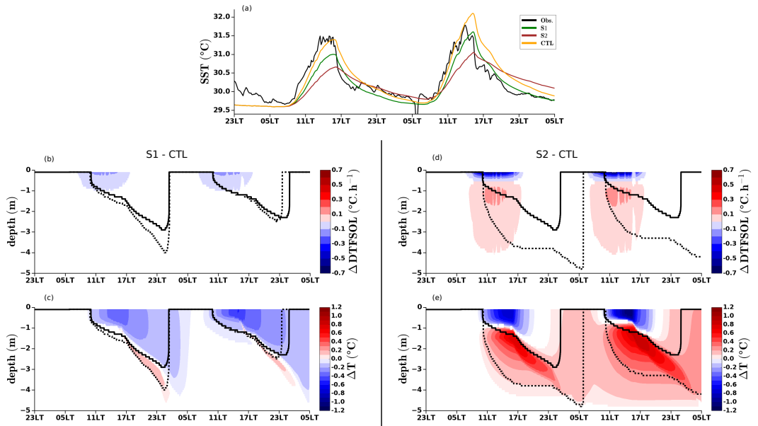
FIGURE 5 (a) Time series of the sea surface temperature (SST), the back line corresponds to the SST monitored at the R/V Revelle with a sea snake and the coloured lines correspond to the sensitivity tests listed in Table 2. Time–depth cross–sections of the difference the volume heat source induced by the absorption of solar radiation (the first term of the right hand side in eq. 2) and temperature between the simulations listed in Table 2 and the reference simulation (CTL). (b), (c) S1 and (d), (e) S2. The thick black contours represent the depth of the DWL for the reference (solid lines) and the test (dashed lines), respectively.
